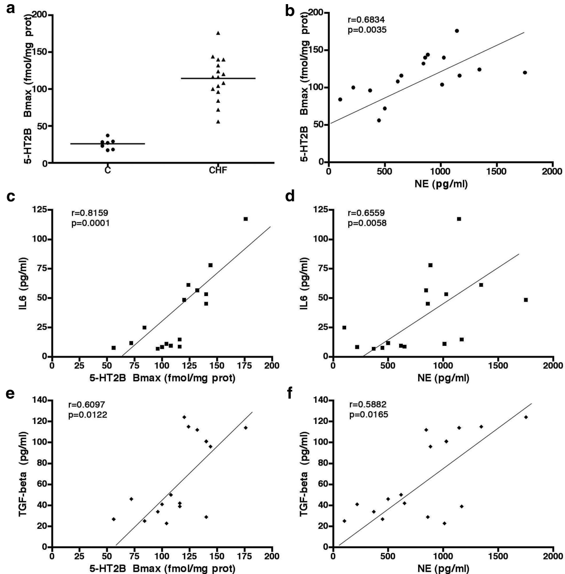
Figure 7. The overexpression of 5-HT 2B Rs observed in human cardiac hypertrophy is correlated with plasma norepinephrine and cytokine levels. a, Expression of 5-HT 2B Rs (Bmax), obtained from biopsies of left ventricles, was found to be significantly elevated and is expressed the average of subepicardial, subendocardial, and midventricle biopsies. Correlations between the cardiac 5-HT 2B R expression levels (in fmol/mg of proteins) and the plasma levels (in pg/mL) of either norepinephrine (b), IL-6 (c), TGF- \beta (e), or TNF- \alpha (Supplemental Figure 4f) are shown. Similarly, correlations between the plasma levels of norepinephrine with either IL-6 (d), TGF- \beta (f), or TNF- \alpha (Supplemental Figure 4g), are given. Probability value (p) and Spearman rank correlation (r) are presented.
