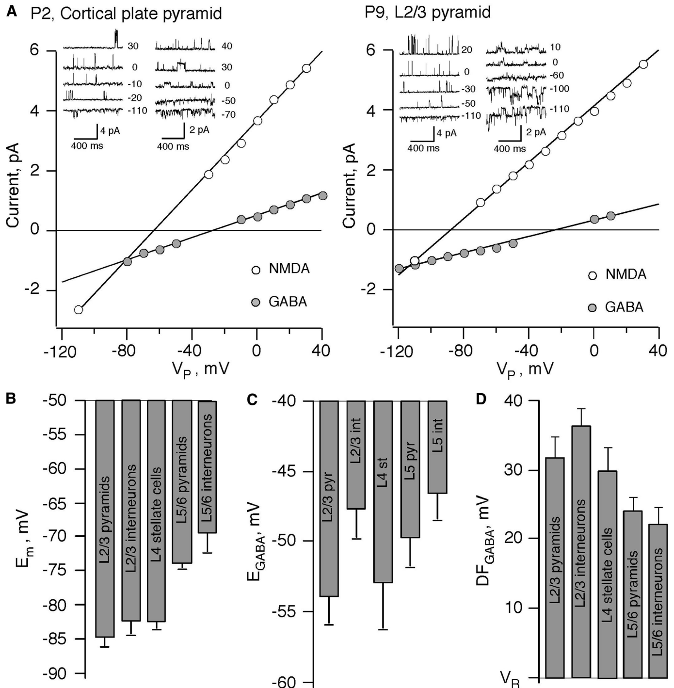
FIG. 1. E_m and E_{GABA} in neonatal neurons measured by cell-attached recordings of single N -methyl-D-aspartate (NMDA)- and GABA-activated channels. A : current-voltage relationships of single NMDA- and GABA-activated channels. Inset : examples of single NMDA ( left ) and GABA ( right ) channel activity at various pipette potentials. Recordings from the same P2 cortical plate pyramidal cell ( left ) and from the same P9 layer 2/3 pyramidal cell ( right ). B : E_m in various cell types and layers of mouse P7–P8 neocortical slices (97 neurons). C : values of E_{GABA} . D : GABA driving force ( DF_{GABA} ) in different cell types and layers of mouse neocortical slices at P7–P8 (59 neurons).
