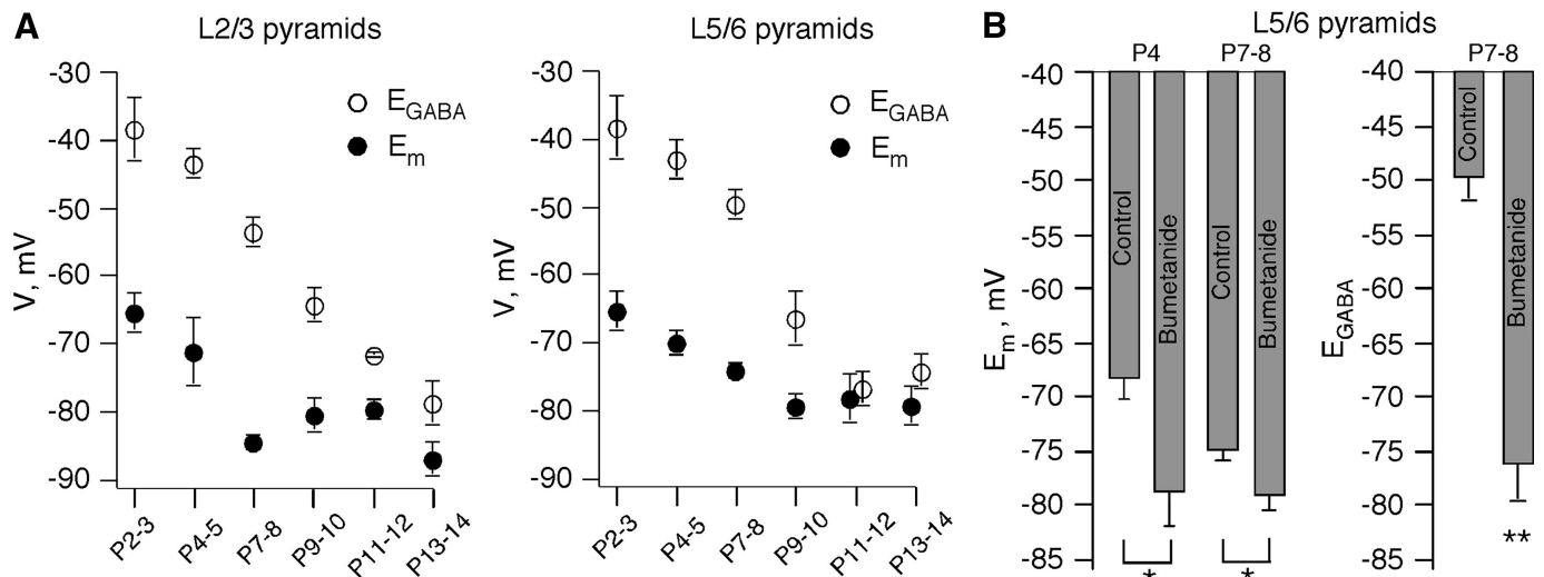
FIG. 2. Developmental profile of E_m and E_{GABA} in pyramidal cells. A : developmental changes in E_m and E_{GABA} in layer 2/3 and 5/6 pyramidal cells (pooled data from 166 cells). B : bumetanide, a NKCC1 chloride co-transporter antagonist, induces hyperpolarization of E_m in P4 (7 cells) and P7/8 layer 5/6 pyramidal cells (15 cells) and strongly decreases E_{GABA} in P7/8 layer 5/6 pyramidal cells (6 cells).
