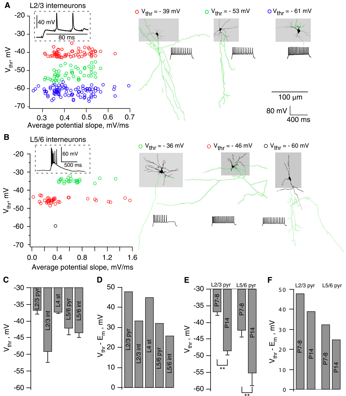
FIG. 3. Action potential threshold ( V_{thr} ) of neonatal neurons. Measurements of V_{thr} in (A) L2/3 and (B) L5/6 interneurons. Cells were excited by random synaptic stimulation (L2/3) or spontaneous oscillations (L5/6). Color codes correspond to the interneurons labeled with biocytin and shown on the right panels. C: V_{thr} in various cell types of P7–P8 neocortex (63 neurons). D: difference between E_m and V_{thr} (relative threshold) in different cell types of P7–P8 neocortex. E: developmental changes in V_{thr} . F: the relative threshold in layer 2/3 and 5/6 pyramidal cells (37 neurons).
