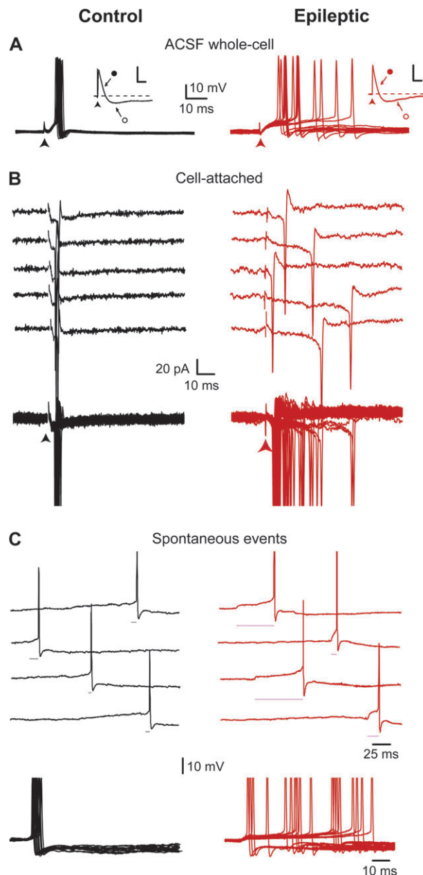
Figure 5. Reduced temporal precision of EPSP-spike coupling in physiological conditions. These experiments were performed in ACSF, in the absence of GABA and NMDA receptor blockers. (A) Superimposed suprathreshold EPSPs recorded in a granule cell from control (black traces) and epileptic (red traces) rats. Note time-locked (SD = 1.0 ms) and jittered spikes (SD = 13.4 ms) in control and epileptic rats, respectively. When EPSP (close circle) is followed by a di-synaptic IPSP (open circle) this shortens EPSP decay and prevents the generation of action potentials both in DGCs from control (black inset) and epileptic (red inset, scale bars: 2 mV, 50 ms) rats. (B) Individuals (top) and superimposed (bottom) loose cell-attached recordings of spiking in response to electrical stimulations in a granule cell from control (black traces) and epileptic (red traces) rats. Note time-locked (SD = 0.6 ms) and jittered spikes (SD = 9.9 ms) in control and epileptic rats, respectively. (C) Continuous recordings of spontaneous suprathreshold EPSPs (top) and superimposed spontaneous suprathreshold EPSPs (bottom, aligned on the rising phase) in a granule cell from control (black traces) and epileptic (red traces) rats. Note that spontaneous EPSPs always trigger spikes from their rising phase in the granule cell from control rat, whereas in the granule cell from epileptic rat spikes are generated either from the rising phase or during the long-lasting plateau of spontaneous EPSPs; EPSP-spike latency is indicated by a horizontal line.
