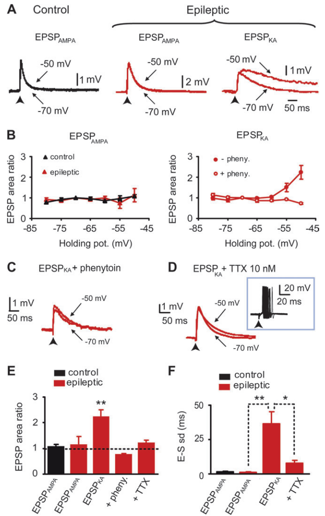
Figure 3. Voltage-dependent amplification of EPSP KAR but not EPSP AMPA via the activation of persistent sodium current. (A) Superimposed average evoked subthreshold EPSP AMPA recorded at threshold holding potential (−50 mV) and at Vrest (−70 mV) in granule cells from control (left, black traces) and epileptic rats (middle, red traces, in the presence of 10 \mu M SYM 2081); superimposed average evoked subthreshold EPSP KAR recorded in a granule cell from an epileptic rat (right, red traces, in the presence of 100 \mu M GYKI 52466). (B) Scatter plot of mean amplification (ratio of EPSP area at −50 vs. −70 mV) versus membrane potential. Note that EPSP AMPA are not amplified with depolarization (left graph), both in control (black triangles, n = 5 cells) and in epileptic rats (red triangles, n = 5 cells); on the contrary, EPSP KAR in epileptic rat (right graph) are significantly amplified with depolarization (filled circles, n = 8 cells). This amplification is completely prevented by phenytoin (100–200 \mu M, open circles, n = 5 cells). (C) Superimposed evoked EPSP KAR recorded in the presence of phenytoin (200 \mu M) in epileptic rat at −50 and −70 mV. Note that the voltage-dependent amplification is completely abolished when persistent sodium current is blocked by phenytoin. (D) Superimposed evoked EPSP KAR recorded in the presence of low concentration of TTX (10 nM) in epileptic rat at −50 and −70 mV. Note that the voltage-dependent amplification is completely abolished when persistent sodium current is blocked by TTX. Trace inset shows that 10 nM TTX does not prevent neuronal firing and increases spike timing reliability. (E) Bar graph of the mean amplification (ratio of EPSP area at −50 vs. −70 mV) for EPSP AMPA in control ( n = 11 cells), EPSP AMPA in SYM 2081 in epileptic rats ( n = 5 cells), EPSP KAR in GYKI 52466 in epileptic rats ( n = 13 cells, **P < 0.01 ), EPSP KAR in the presence of phenytoin in epileptic rats ( n = 5 cells), and EPSP KAR in the presence of 10 nM TTX in epileptic rats ( n = 6 cells). (F) Bar graph of EPSP-spike latency SD for EPSP AMPA in control ( n = 20 cells), EPSP AMPA in SYM 2081 in epileptic rats ( n = 5 cells), EPSP KAR in GYKI 52466 in epileptic rats ( n = 17 cells, **P < 0.01 ), and EPSP KAR in the presence of 10 nM TTX in epileptic rats ( n = 7 cells, *P < 0.05 ).
