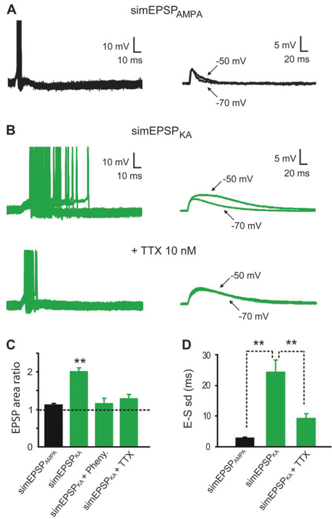
Figure 4. SimEPSP K A generate spike with low temporal precision in granule cells from control rats. Simulated EPSPs (simEPSPs) with different kinetics were generated through somatic current injections to mimic synaptic AMPAR or KAR-mediated EPSPs in granule cells from control rats. (A) simEPSP AMPA (right, -50 mV) evoked time-locked spikes (left superimposed traces) and were not significantly amplified with depolarization from -70 mV to -50 mV (right, superimposed average traces). (B) simEPSP K A (upper right, -50 mV) generated late and highly variable spikes (upper left superimposed traces) and showed a significant amplification with depolarization to -50 mV (upper right superimposed traces) in a granule cells from a control rat. In the presence of TTX 10 nM, EPSP-spike coupling temporal precision was significantly restored (bottom left traces) and voltage-dependent amplification was abolished (bottom right traces). (C) Bar graph of mean amplification (ratio of simEPSP area at -50 vs. -70 mV) of simEPSP AMPA (black column, n = 7 cells), simEPSP K A (green column, n = 18 cells, P < 0.01), simEPSP K A in the presence of phenytoin (100–200 μM, n = 7 cells) and simEPSP K A in the presence of TTX (10 nM, n = 9 cells) in granule cells from control rats. (D) Bar graph of EPSP-spike latency standard deviation (E-S SD) of simEPSP AMPA (black column, n = 8 cells), simEPSP K A (green column, n = 18 cells, ** P < 0.01), and simEPSP K A in the presence of TTX (10 nM, n = 9 cells, ** P < 0.01) in granule cells from control rats.
