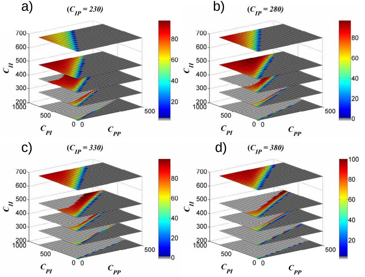
Figure 6: Joint influence of glutamatergic and GABAergic connections (i.e., C_{PP}, C_{PI}, C_{IP}, C_{II} parameters) on the resonance frequency of the output signal. Each 3D plot corresponds to a set of C_{PP}, C_{PI}, C_{II} parameters at a fixed C_{IP} value indicated on the top of each figure. As before, stable and unstable regions are shown by dark and light grey, respectively. Resonance regions in the 2D planes (i.e. C_{PP} - C_{PI} planes) expand and rotate anti-clockwise when C_{II} increases. This movement decreases the resonance frequency as a function of C_{II} . When too much pronounced, the decrease or increase in C_{II} value leads to disappearance of the resonance region or limits the maximum reachable resonance frequency, respectively. C_{IP} has opposite effects on resonance characteristics of the output signal, compared to C_{II} .
