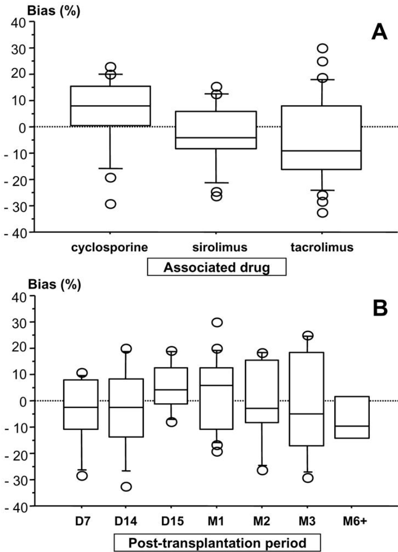
Figure 2 Bias of the Bayesian estimates of MPA AUC_{0-12h} obtained using the 20 min-1h-3h sampling schedule with respect to the “true”, trapezoidal AUC_{0-12h} sorted out by: A) associated immunosuppressant; and B) post-transplantation periods.
