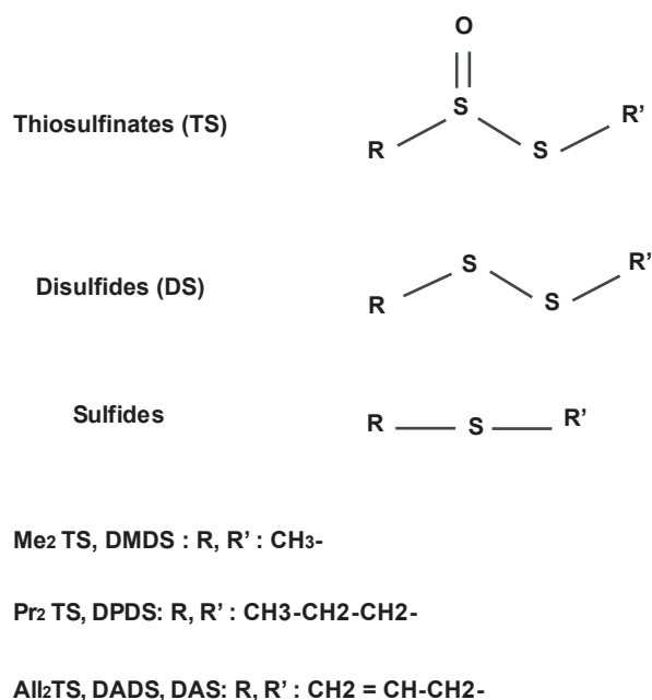
Figure 1 Structure of thiosulfinates and sulfides used in this study. Abbreviations: DADS, Diallyl disulfide; DAS, dialylsulfide; All 2 TS, diallyl thiosulfinate; DMDS, dimethyl disulfide; Me 2 TS, dimethyl thiosulfinate; DPDS, dipropyl disulfide; Pr 2 TS, dipropyl thiosulfinate.
