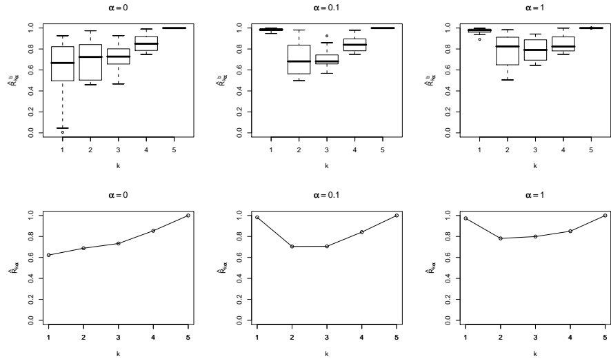
Figure 3: Boxplots of the \hat{R}_{k,\alpha}^{(b)} 's values (above) and plots of \hat{R}_{k,\alpha} (below) versus k , for \alpha = 0, 0.1 and 1.
