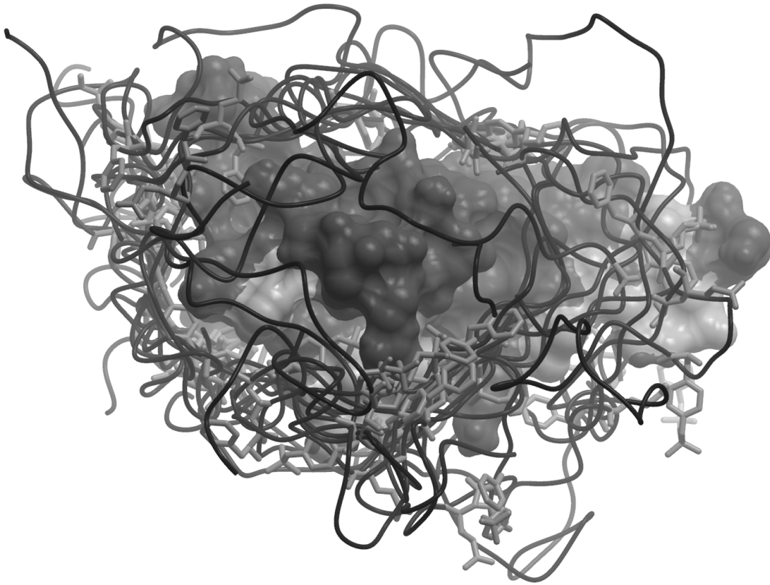
Figure 13. Flexible docking. Some snapshots of the flexible search of ECD1 around the rigid structure of CXCL8 monomer are shown.
