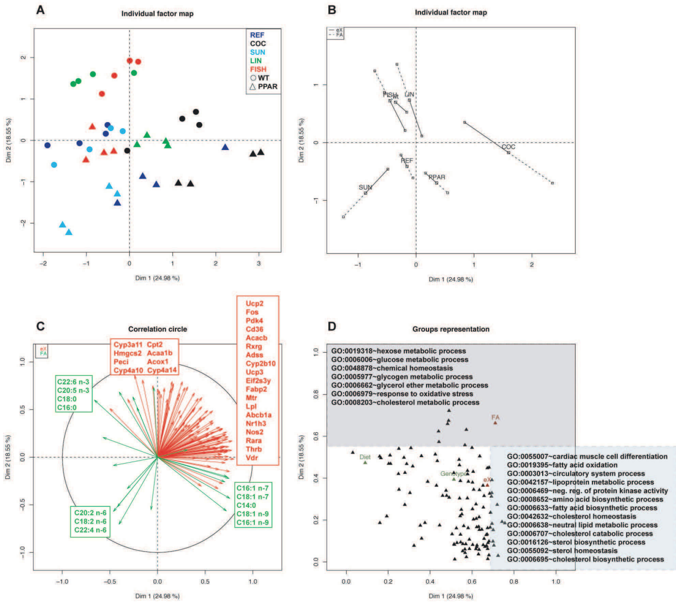
Figure 8 Multi-way nutriment data set: MFA approach provides findings in accordance with those found by specialists. A and B. Individual factor maps show partition of the mice according to Diet and Genotype. Mice fed the COC diet (black circles and triangles) are separated from the other mice on PC1. PPAR deficient mice (triangles, PPAR) are separated from wild-type mice (circles, WT) on PC2. C. Variables representation. The genes and FAs most correlated to each principal component are named. Mice from both genotype displayed specific accumulations of FA families. Mice fed the SUN diet had enriched proportion of n-6 FAs, those fed the LIN and FISH diets are particularly related to n-3 FAs. Mice fed the COC diet preferentially accumulate mono-unsaturated FAs in their livers. Genes most correlated with PC2 are PPAR target genes (Peci, Cyp4a10, Cyp4a14, Acox1, Acaa1b, Hmgcs2, Cpt2) or genes involved in hepatic detoxification (Cyp3a11). D. Enriched GO terms ( p -value < 0.05) are projected on the Groups scatter-plot, the most correlated to each PC are named. Annotations related to PC1 and PC2 are respectively linked to FA and glucose metabolism. The GO term 'cardiac muscle cell differentiation' (GO:0055007) is enriched by class II nuclear receptors (retinoid \times receptors and retinoic acid receptors) which are also key regulators of lipid metabolism.
