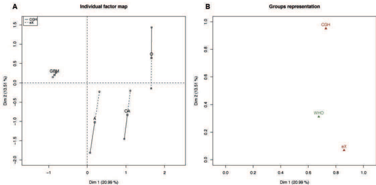
Figure 3 Multi-way glioma data set: Characteristics of glioblastoma are linked to CGH and expression data whereas characteristics of oligodendrogliomas are mostly related to CGH data. The partial representation of the mean individuals (CGH and eX) for each WHO tumor type (A) and the group representation (B) are displayed. (A) The balanced representation of each category is located in the exact barycenter of the points summarizing partial points of view (CGH; linked by plain line and eX; linked by dot line). The projection of the partial representations for each category (CGH and eX for oligodendrogliomas, astrocytomas, oligoastrocytomas and glioblastomas) onto PC1 are very close; the partition of the tumors into WHO classification is thus shared by the genome and the transcriptome. On PC2, all the mean individuals from the partial expression representation (eX) are located around the origin. It is not the case for the genomic one (CGH). PC2 is therefore specific to the genomic point of view and is not shared by the expressional one. This is confirmed by analyzing the group representation (B): projection of the CGH and eX groups are closed along PC1 but only the one of CGH have a value close to 1 on PC2.
