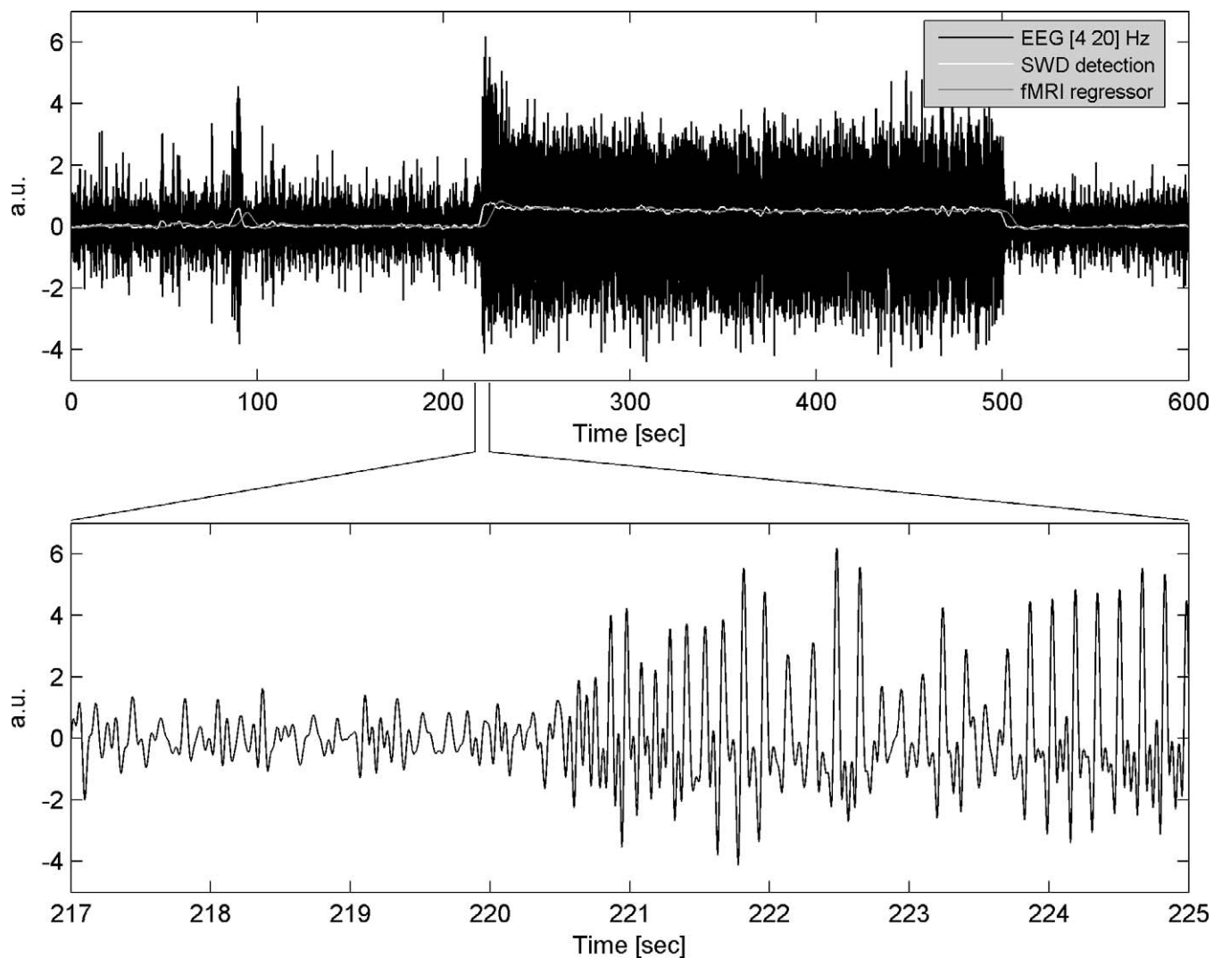
Figure 1. EEG Preprocessing
