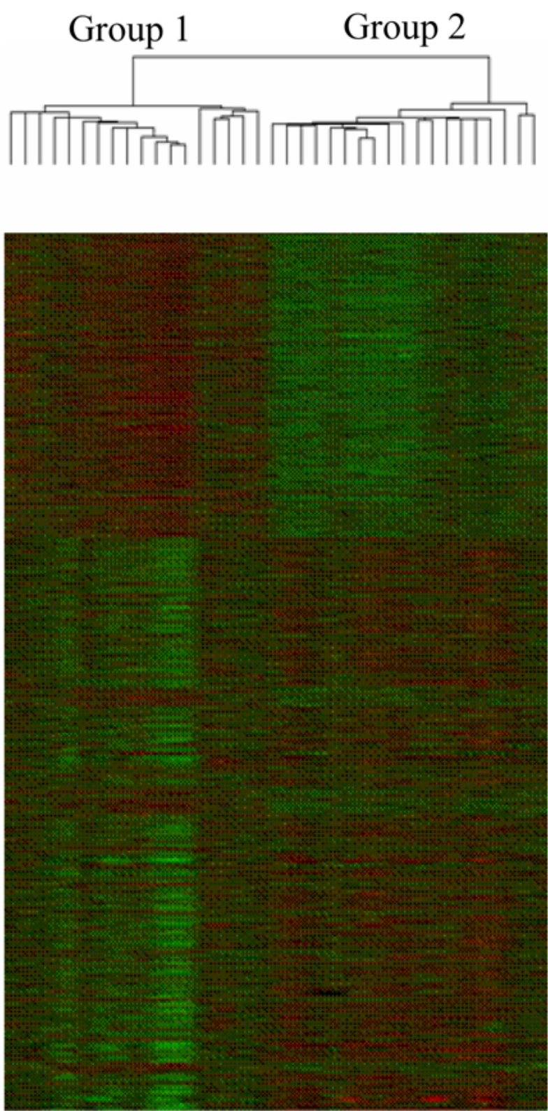
Figure 1 Hierarchical cluster analysis of BPH samples as visualized with Tree view software: two main groups of 18 and 19 samples, respectively, are observed.
