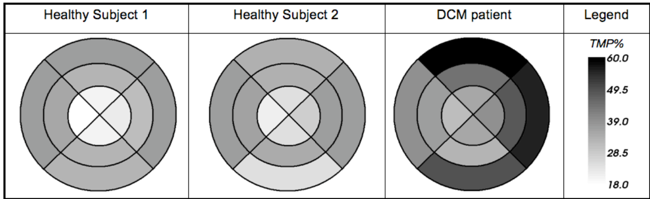
i46 i47 Figure 15: Bull's eye representation of the mechanical activity peak time expressed as a percentage of the RR-interval ( TMP\% ) for the two i48 healthy subjects and the pathologic patient. These values are high for the anterior and lateral segments of the DCM patient.
