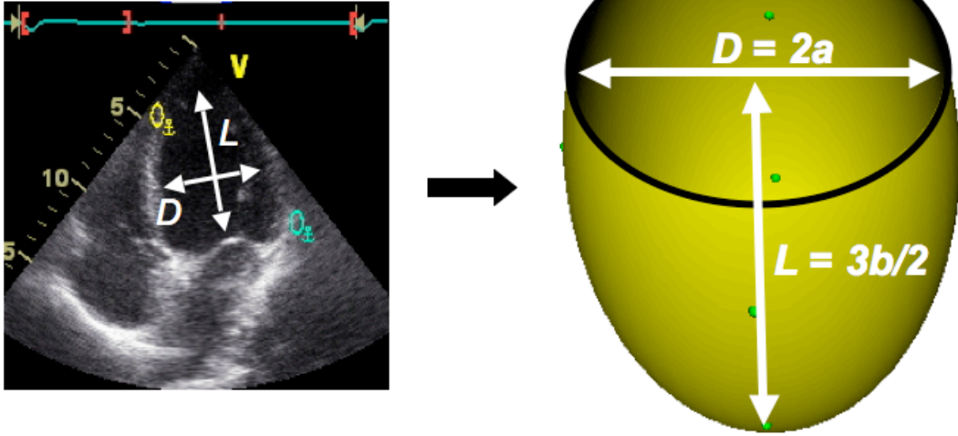
Figure 9: Ellipsoidal model dimensions obtained from echocardiographic measures: a and b are respectively the minor and major axis sizes.
