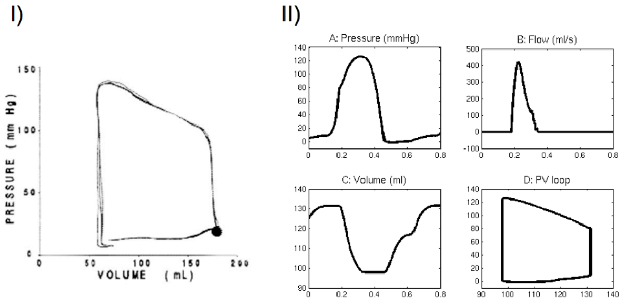
.62 Figure 6: I) Stable resting left ventricular pressure-volume loop acquired from a human. The figure has been reproduced with permission from .63 [65], II) Model simulation of ventricular hemodynamic variables for one beat: A) intra-ventricular pressure B) aortic flow C) volume D) .64 pressure-volume loop.
