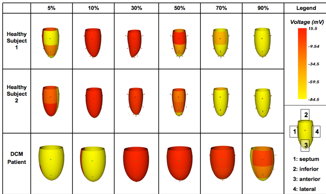
11 12 Figure 12: Contraction of the electromechanical model for the two healthy subjects and the pathologic patient. The color legend corresponds to 13 the electrical state of each segment and is expressed in mV. The orientation of the ventricular model is depicted in the lower right panel of the 14 figure.
