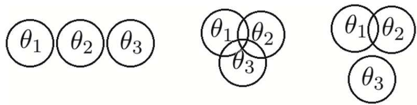
Fig. 3 Considering the frame of discernment \theta = \{\theta_1, \theta_2, \theta_3\} , the figure represents, from left to right, the Venn diagram of the constrained, the free and a hybrid model (in which \theta_3 is incompatible with the other two hypotheses). A non-empty intersection between circles means the corresponding hypotheses are compatible.
