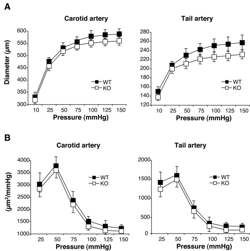
Figure 1 Passive diameter (A) and cross-sectional compliances (B) of carotid and tail caudal arteries from wild type (WT) and Notch3 -/- (KO) mice (MEAN ± SEM, n=12 WT and 9 KO); NS, KO versus WT.
