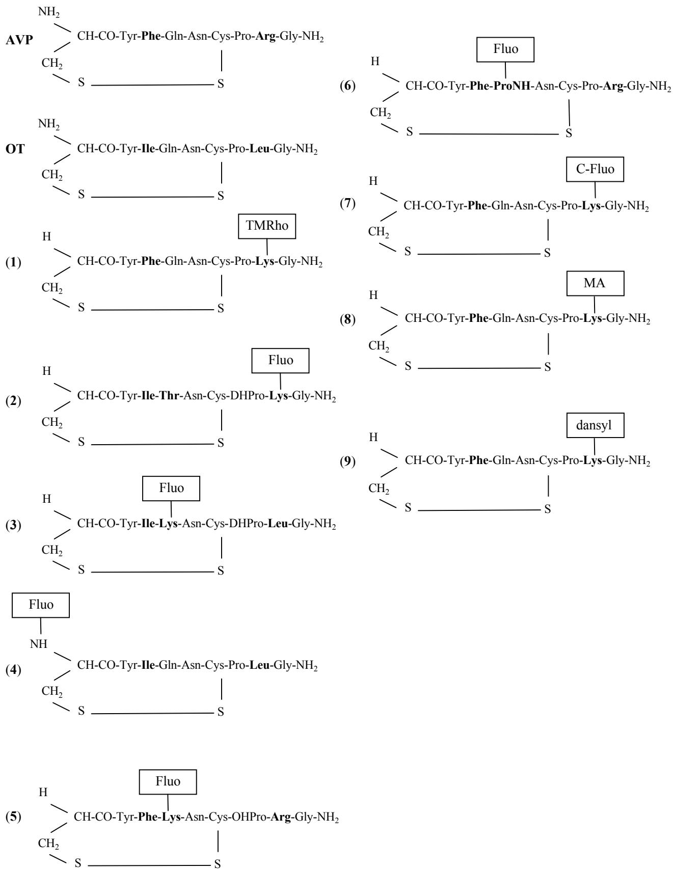
Figure 1: fluorescent agonist analogs of AVP/OT.
