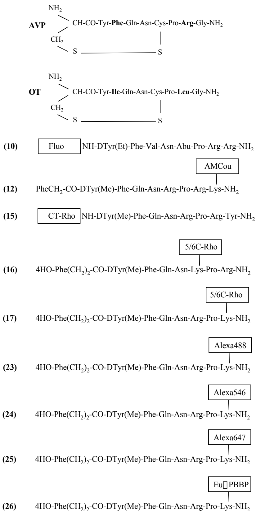
Figure 4: fluorescent linear antagonist analogs of AVP/OT.
