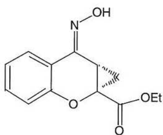
(-)-CPCCOEt
