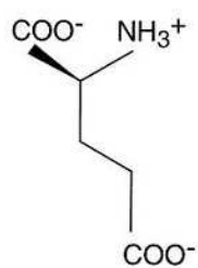
L-Glutamate
