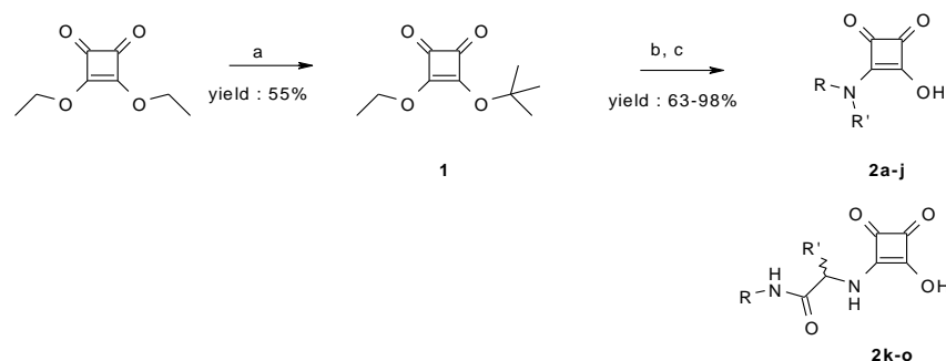
Scheme 1. Reaction conditions : a. t-BuOK, 1M in THF (1eq.), THF, 4°C ; b. RR'NH, NEt 3 , EtOH, r.t.; c. TFA/dichloromethane (1/1 v/v), 4°C.
