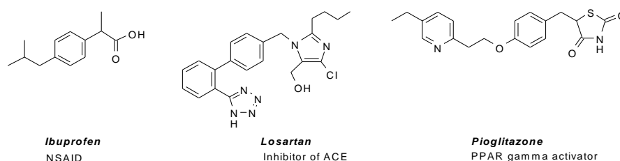
Figure 4. Examples of structures of acidic drug molecules.
