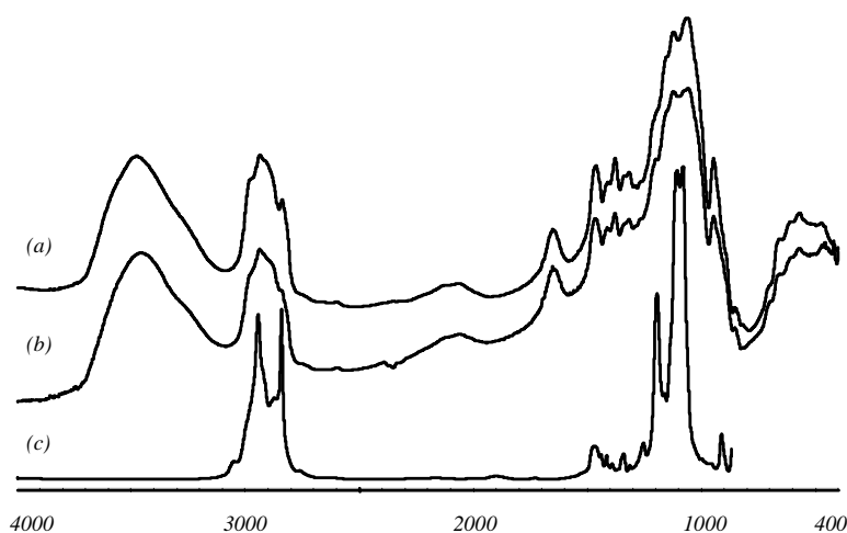
Figure 2. FTIR spectra: (a) HPMC, (b) siliated-HPMC and (c) 3-glycidoxipropyltrimethoxysilane.
