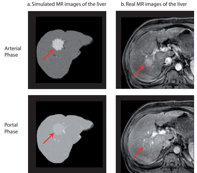
Fig. 4. Comparison between simulated (a) and real (b) Dynamic Contrast-Enhanced MR images of the liver. Acquisition conditions: 3D Gradient Echo sequence 3T ( T_E = 1.36ms , T_R = 2.75ms , Flip\ Angle = 10^\circ , Slice\ Thickness = 4mm ); Contrast agent: Gd-DOTA; Up : arterial phase. Down : portal phase. Note: red arrows indicate the tumor.
