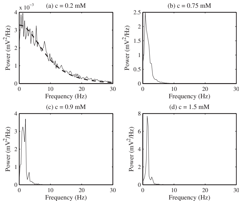
FIG. 7. The power spectra of simulated h_e signals in different drug concentrations. Each power spectrum is calculated by averaging 20 power spectra of consecutive 2.56 s h_e epochs (i.e., 51.2 s). (a) In very low drug concentration ( c=0.2 mM), the power spectrum extends to high frequency terms. The eigenspectrum (dashed line) corresponding to this drug concentration is a descending function that is reminiscent of the background spectrum of a real EEG signal in the waking period. (b) Appearance of slow waves ( c=0.75 mM), increases the energy of the slow delta band in the power spectrum. (c) Increasing the rate of slow waves ( c=0.9 mM) increases the energy of the fast delta band in the power spectrum. (d) Regular switching between up and down state ( c=1.5 mM) narrows the h_e spectrum in the fast delta band.
