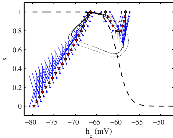
FIG. 12. (Color online) s, h_e isoclines and a 20 s (s, h_e) trajectory corresponding to burst suppression in high anesthetic drug concentration ( c=1.8, B=0.14, \theta_s=-60 ). The intersection of the two isoclines is very close to the saddle point of the h_e isocline so (s, h_e) trajectory has the possibility of short-time traveling from down to up state.
