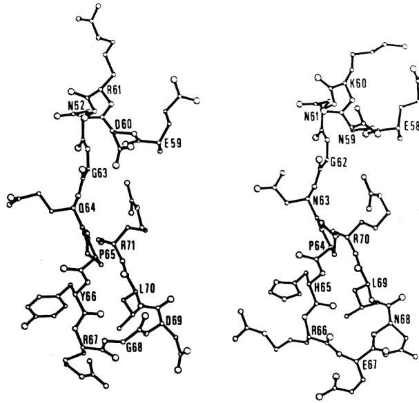
Figure 2. View of the putative receptor binding site of bovine angiogenin (Left) and human angiogenin (Right). Reproduced with permission from [46] (Copyright 1995, Proc. Natl. Acad. Sci. USA).
