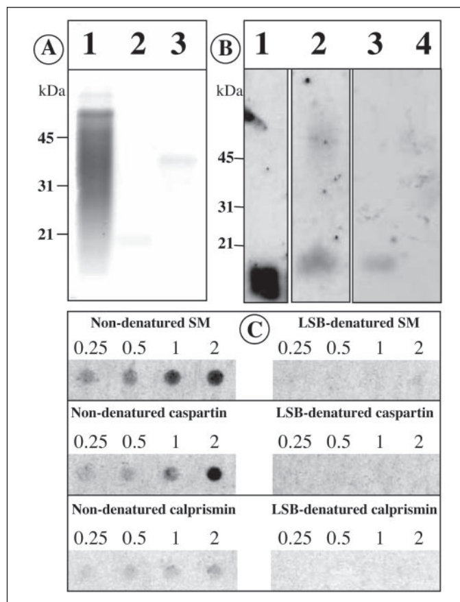
FIGURE 5. Calcium-binding properties of the acetic acid-soluble prism matrix (SM), of caspartin and of calprisin. A, staining with the carbocyanine dye Stains-All. Lane 1, soluble matrix (10 μg); lane 2, caspartin (~5 μg); lane 3, calprisin (~5 μg). B, 45 Ca-binding overlay test. Lane 1, calmodulin (2 μg); lane 2, soluble matrix (30 μg); lane 3, caspartin (20 μg); lane 4, calprisin (20 μg). C, 45 Ca-binding overlay test on dot blots of the soluble matrix, of caspartin and of calprisin in denaturing (in the presence of Laemmli sample buffer (LSB)) and nondenaturing conditions. Different amounts were tested (0.25, 0.5, 1, and 2 μg). The soluble matrix exhibits the strongest calcium binding activity, and calprisin exhibits the lowest. Laemmli-treated samples have lost their ability to bind calcium.
