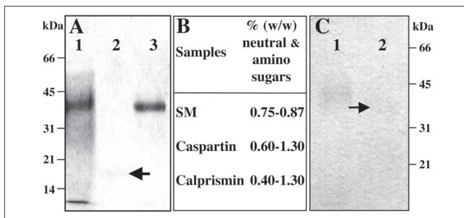
FIGURE 6. Glycosylation study of the acetic acid-soluble prism matrix (SM), of caspartin, and of calprisin. A, staining with Alcian blue. Lane 1, soluble matrix (20 \mu g); lane 2, caspartin (10 \mu g); lane 3, calprisin (10 \mu g). The soluble matrix and calprisin stain well with Alcian blue, whereas caspartin, localized by the arrow, hardly stains. B, determination of the amount of neutral and amino sugars (in percentage of dry weight) after hydrolysis of the samples with trifluoroacetic acid and analysis by high performance anion exchange-pulsed amperometric detection. Batches 1 and 2 were used for the analysis. The three samples are characterized by low amounts of neutral and amino sugars. C, staining of calprisin with Alcian blue before (lane 1; 10 \mu g) and after (lane 2; 10 \mu g) an enzymatic deglycosylation. A decrease of the staining can be observed after the deglycosylation treatment. The arrow localizes the deglycosylated calprisin.
