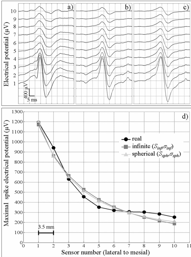
Fig. 7. A simulation example of a transient epileptiform activity (spike). (a) Real depth-EEG signals were recorded by an intracerebral electrode implanted in the left middle temporal gyrus (from mesial - top - to lateral - bottom - sensors). Simulated signals obtained from the extended source model (patch of neocortex located in the left temporal lobe) in which surface and conductivity parameters ( S, \sigma ) are set to values corresponding to minimal RMSE (see Fig. 6), for infinite volume conductor model (b) and for 3-shell spherical head model (c). (d) Comparison of real (circle) and simulated voltages along the intracerebral electrode for both the infinite model (square) and the spherical model (triangle). Voltage estimator corresponds to the spike maximal potential.
