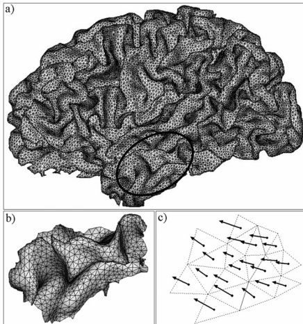
Fig. 2. (a) A triangular mesh of the inner brain surface (grey-white matter interface) is built from the segmentation of 3D MRI data ( \sim 80000 triangles per hemisphere). In the extended source model, a surface element of neocortex is considered, as exemplified in the temporal lobe (ellipse). (b) This element of neocortex is composed of small elementary triangles ( \sim 1 \text{ mm}^2 per triangle). Each triangle is assumed to represent a neuronal population. (c) The electrical contribution of each neuronal population is represented by an elementary current dipole which is placed at the barycentre of the triangle and which is oriented orthogonally to triangle surface. The moment of each elementary dipole is weighted by both the triangle area and the population time-varying field activity.
