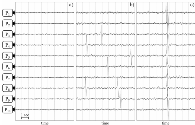
Fig. 5. Influence of the coupling strength in a network of ten interconnected neuronal populations. All connections are bidirectional with identical strength K . (a) For null coupling ( K=0 ), resulting signals correspond to normal background activity. (b) The increase of parameter K leads the model to generate sporadic spikes which appear randomly and independently from one population to another. (c) For high K values, synchronization is enhanced and single spikes that involve jointly all populations are produced.
