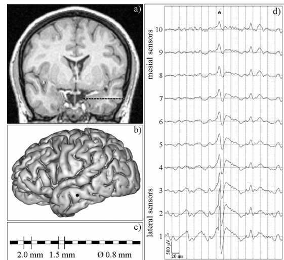
Fig. 3. An example of SEEG exploration. For simplicity, only one intracerebral electrode is represented. However, during presurgical evaluation, the usual procedure uses 5 to 10 electrodes to explore brain regions that are supposed to be involved in epileptic activity. (a) MRI data of a patient suffering from lateral temporal lobe epilepsy. An intracerebral electrode is implanted in the left middle temporal gyrus, orthogonally to the sagittal plane. (b) Lateral view of the cortex, with surgical entrance point of the electrode in the left middle temporal gyrus. (c) Along each electrode, 10 to 15 cylindrical sensors (length: 2 \text{ mm} , diameter: 0.8 \text{ mm} , 1.5 \text{ mm} apart) record signals from mesial (deep) and from lateral neocortical (middle temporal gyrus, superior temporal gyrus) structures. (d) An example of depth-EEG signals recorded by a 10-sensor intracerebral electrode, from mesial sensors (#7-10) to lateral, i.e. neocortical, sensors (#1-4). Asterisk indicates an interictal epileptic spike with maximal amplitude at lateral sensors and progressive amplitude decrease from lateral to mesial sensors.
