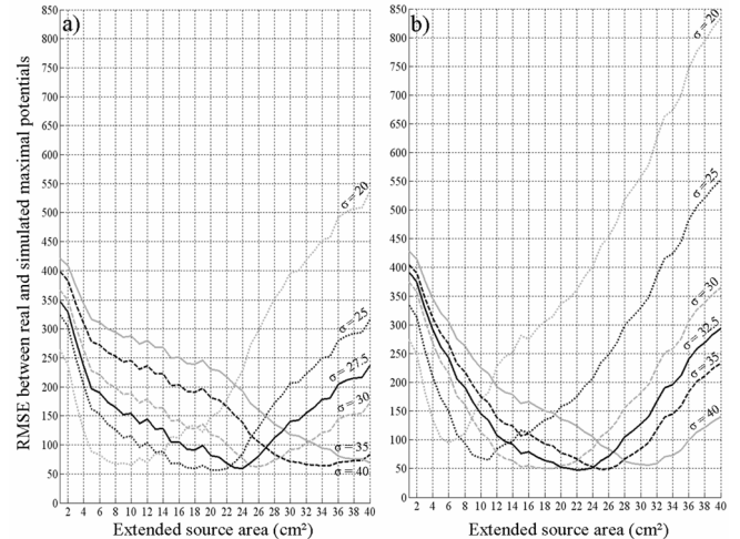
Fig. 6. Root mean square error (RMSE) computed between simulated and real spike maximal potentials, with respect to variations of parameters S (extended source area) and \sigma (brain conductivity), for both volume conductor models. (a) In the infinite case, a global RMSE minimum ( RMSE_{inf} = 56.67 ) was obtained for S_{inf} = 20 \text{ cm}^2 and \sigma_{inf} = 25 \times 10^{-5} \text{ S/mm} (black dotted line). (b) In the spherical case, the global RMSE minimum ( RMSE_{sph} = 47.32 ) corresponded to S_{sph} = 22 \text{ cm}^2 and \sigma_{sph} = 32.5 \times 10^{-5} \text{ S/mm} (black solid line).
