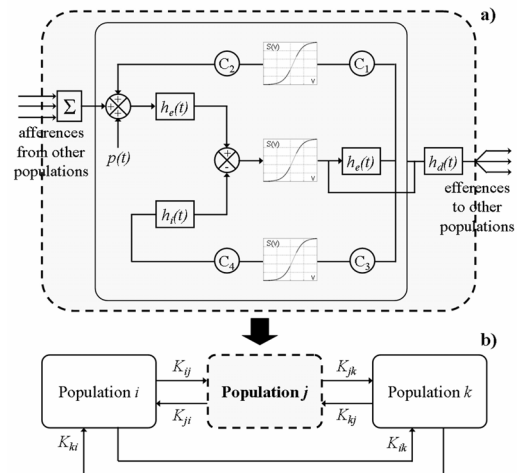
Fig. 1. Structure of the model of multiple coupled neuronal populations. (a) Elementary model for a given population j within (b) the multiple coupled population model. Appropriate setting of parameters K_{ij} allows for neuronal populations to be unidirectionally and/or bidirectionally coupled. Each population of neurons produces a signal corresponding to local field activity.
