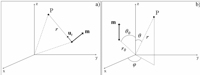
Fig. 4. Coordinate systems. (a) Coordinate system for a dipole in the infinite volume conductor model. (b) Coordinate system for a dipole in the 3-shell spherical head model; particular case of a dipole of moment \mathbf{m} located at (r_0, \theta_0, 0) and parallel to the z -axis.
