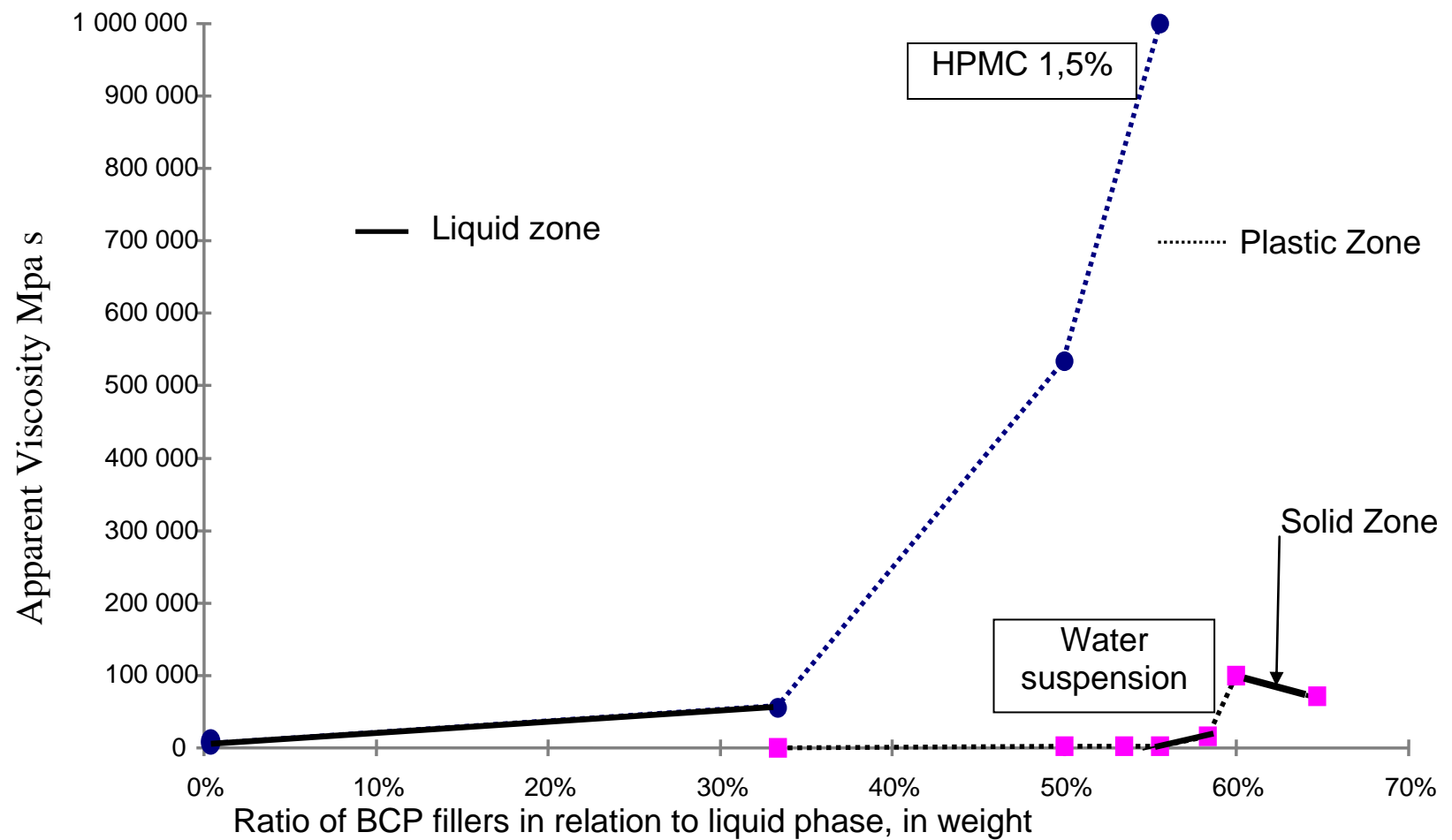
Figure 1. Apparent viscosity (Brookfield RDV11, 1 rpm) of two calcium-phosphate water suspensions as a function of BCP ratio in weight. One of the suspensions was performed only with water, and the other with aqueous polymer solution (1.5% of HPMC in water w/w).
