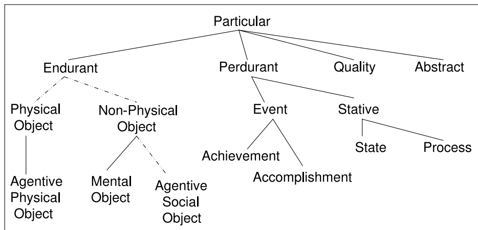
Figure 2: An excerpt from DOLCE's top-level taxonomy
