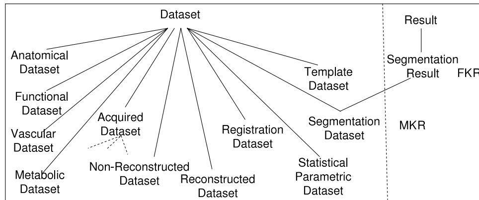
Figure 9: An excerpt from the Dataset top-level taxonomy
