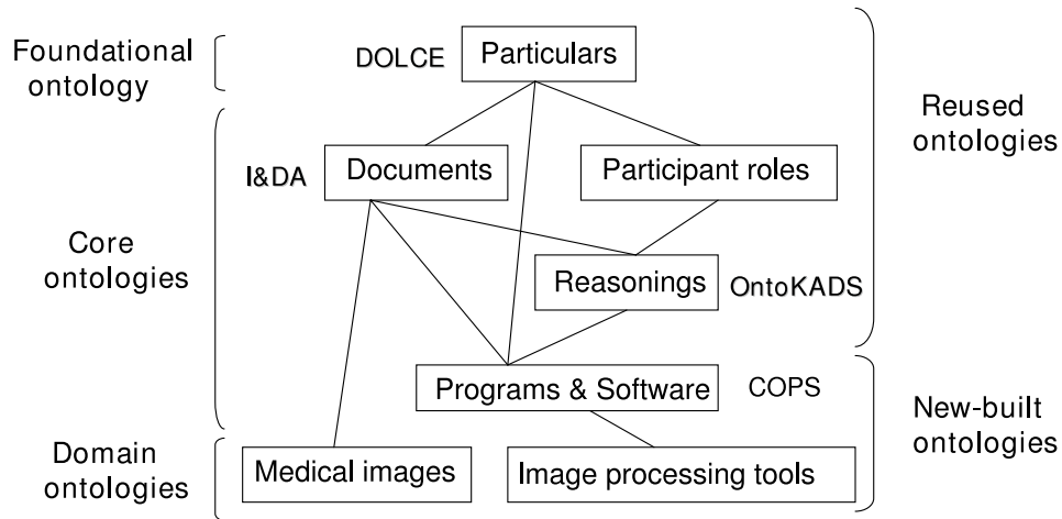
Figure 1: Main ontologies composing OntoNeuroBase kernel. A descending link between two ontologies O_1 and O_2 means that concepts and relations of O_2 specialize concepts and relations of O_1 .
