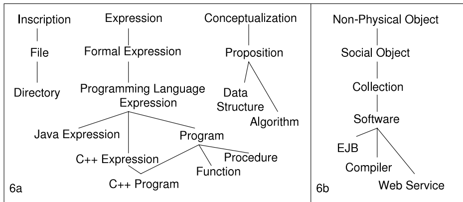
Figure 6: I&DA structures for various entities linked to the notion of Program (6a) and Software (6b).
