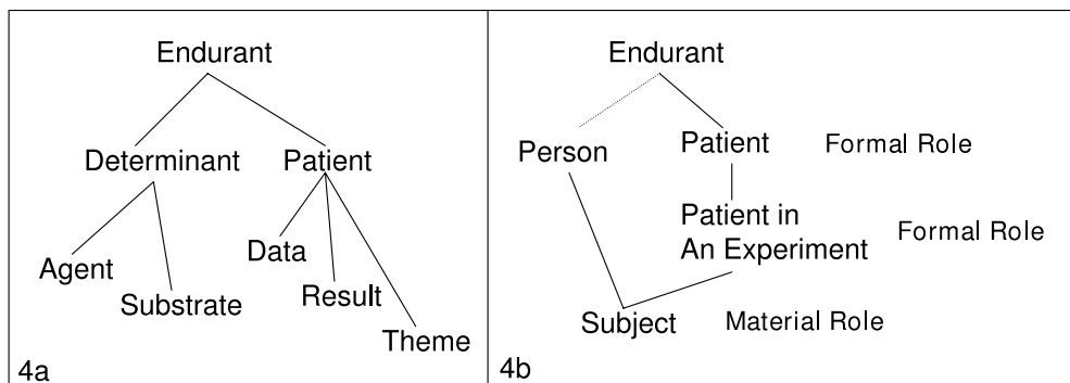
Figure 4: Participant roles (4a); Definition of Material Roles by specialization of Formal Roles (4b)
