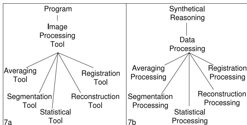
Figure 7: An image processing tool sub-ontology (7a) and a data processing sub-ontology (7b)
