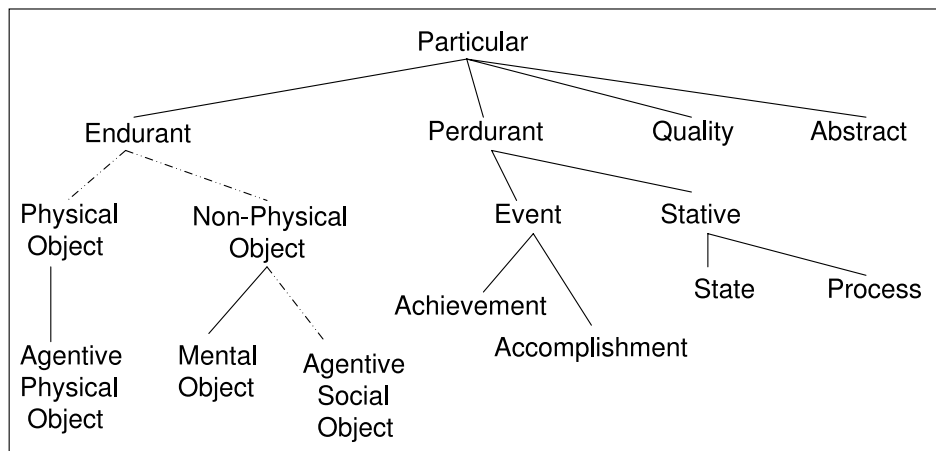
Figure 2: An excerpt from DOLCE's top-level taxonomy
