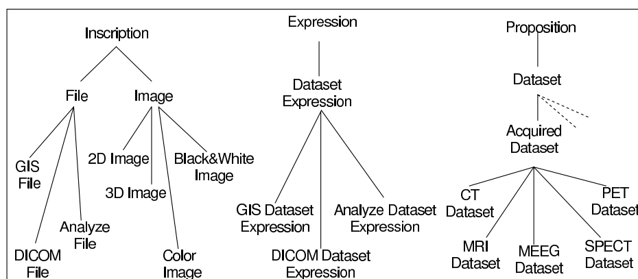
Figure 8: An excerpt from the Dataset ontology
