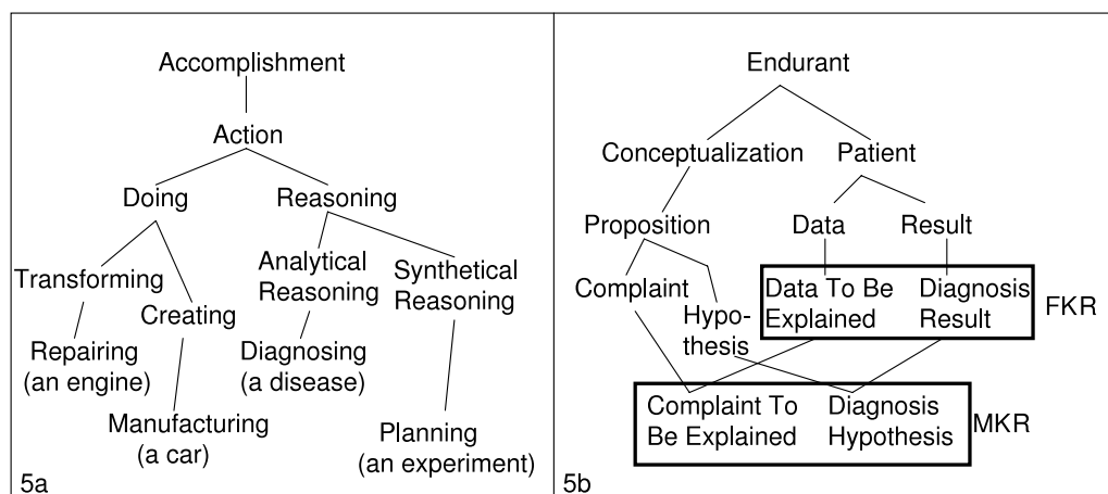
Figure 5: OntoKADS ontology of Actions (5a); Definition of Material Knowledge Roles (MKR) by specialization of Formal Knowledge Roles (FKR)
