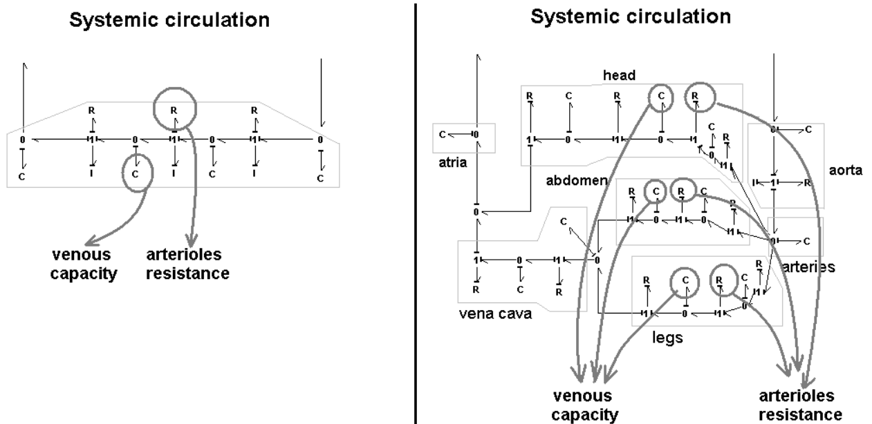
Figure 8. Elements of the Bond Graph model that are under the influence of the ANS model on the simple circulatory model (a) and the more detailed model (b).
