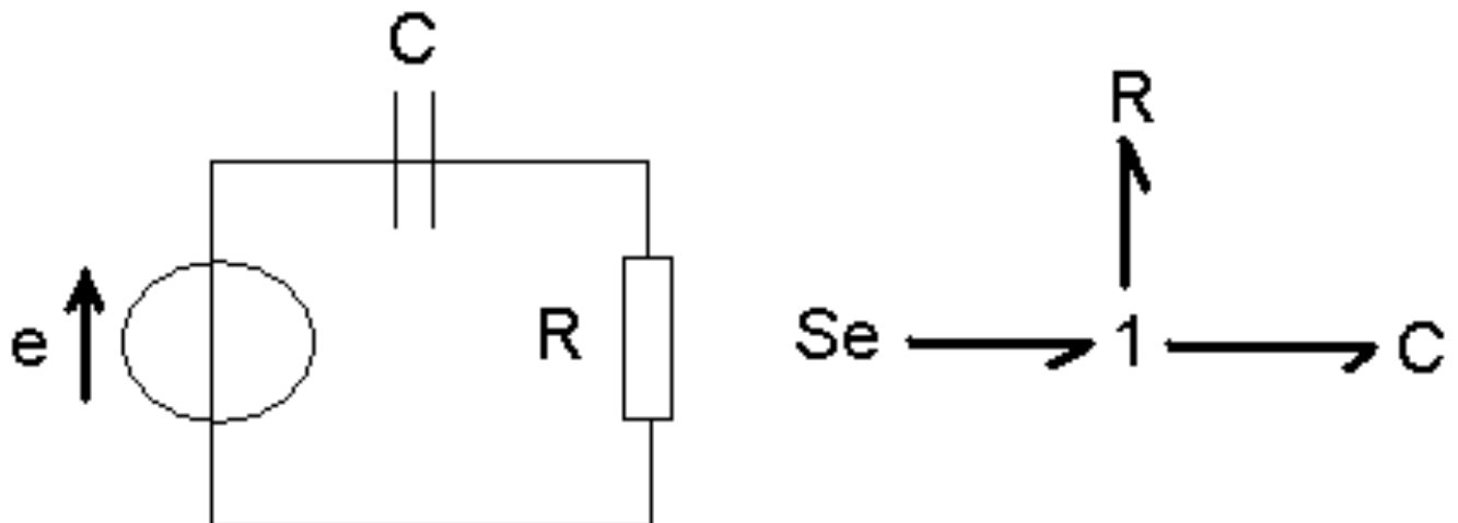
Figure 1. Example of a simple Bond Graph model of an RC circuit.
