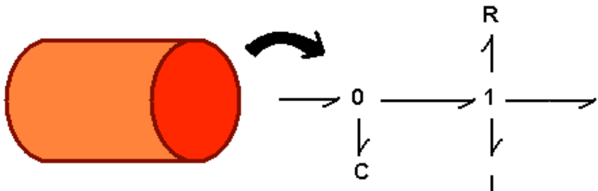
Figure 4. Bond Graph model of a vessel segment.
