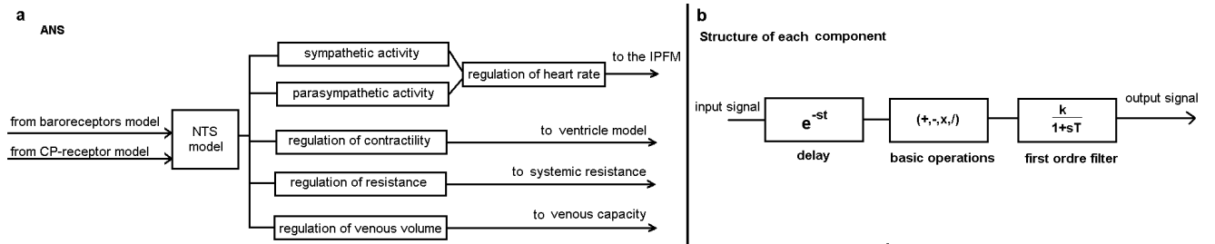
Figure 7. a) components of the ANS model b) structure of each ANS regulation component.
