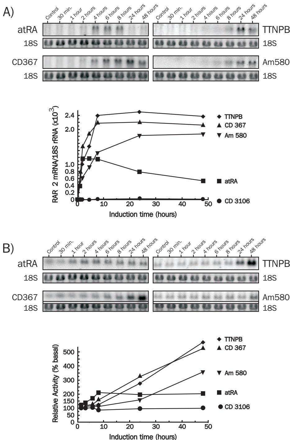
Figure 5 Expression of RAR \beta and of CRABP II in murine P19 cells treated with different ligands of the retinoic acid receptor. A) Time-course analysis of RAR \beta transcripts. RAR \beta transcripts were assayed by Northern blotting (upper panel) and quantified by densitometry. A more rigorous measurement of each time point was carried out by submitting the same sample to real time PCR quantification, using, as for the Northern blot analysis, 18S RNA as an internal standard. All results are expressed relative to RAR \beta level of expression in non stimulated cells. Representative autoradiograms and PCR quantification are shown here, but have carried out 3 times with similar results. B) Time-course analysis of CRABP II transcripts. Assays were carried out as described in A), setting the reference (non stimulated cells) to 100%. Retinoid concentrations were as in Figure 3.
