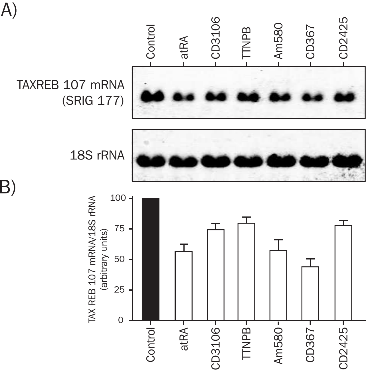
Figure 4 Expression of TAXREB107 mRNA in HeLa cells treated with different ligands of the retinoic acid receptor. HeLa cells were treated with the different ligands for 4 hours. Total RNA (20 µg) was probed sequentially with fluorescein-labeled partial human TAXREB cDNA and 18S rRNA probes. Blots were quantified using a Storm™ apparatus. Values for the TAXREB transcript were normalized to the 18S rRNA level. A) Upper panel: TAXREB107 transcript in HeLa cells treated with various retinoids. Lower panel: 18S rRNA. B) Quantification of TAXREB107 expression. Results are presented as the mean +/- S.E.M. of three different experiments. Retinoid concentrations were as in Figure 3.
