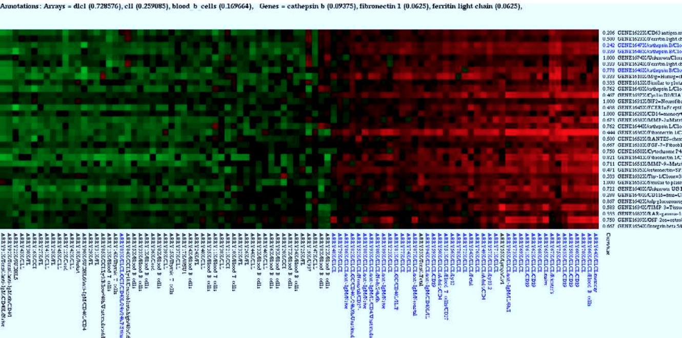
Figure 6 A cluster of genes over-expressed in the DLCL tumors obtained from the lymphoma data with T_{cor} = 0.80 and T_{curv} = 0.24
