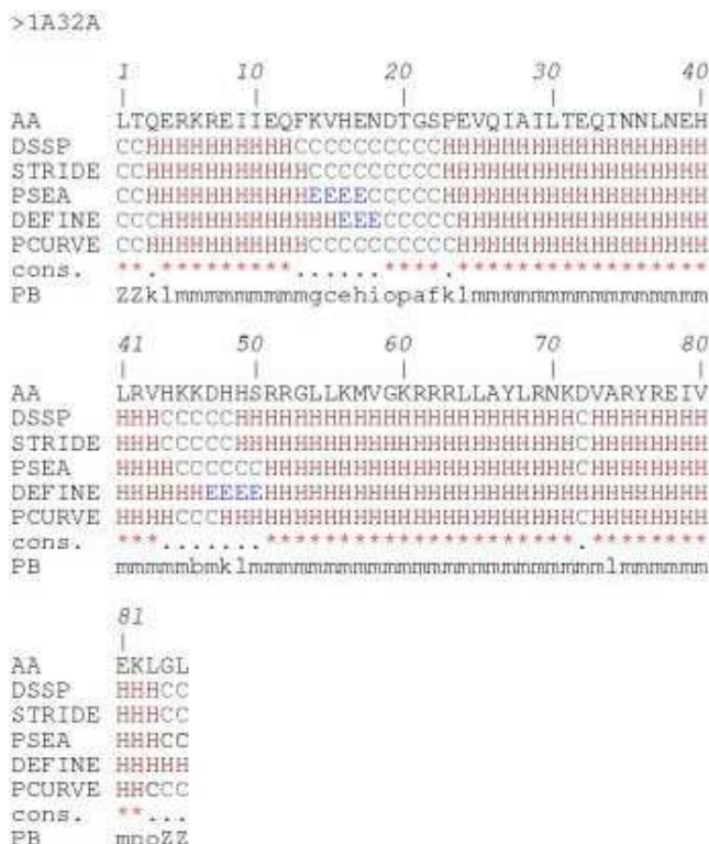
Figure 2 Comparison of methods for secondary structure assignment. Example of 5 assignments for the ribosomal protein S15 from Bacillus Stearotherophilus (PDB code 1A32). The figure shows the amino acid sequence (AA), the secondary structure assignments by (DSSP), (STRIDE), (PSEA), (DEFINE), (PCURVE) with 'H' for the \alpha -helix, 'E' for the \beta -strand and 'C' for the coil, (cons.) is a simple consensus with a star (*) if the five methods agree or a dot (.) if they do not, (PB) is the Protein Block assignment with ZZ for the extremities (not assigned, i.e., the PB is centered on the central residue).
