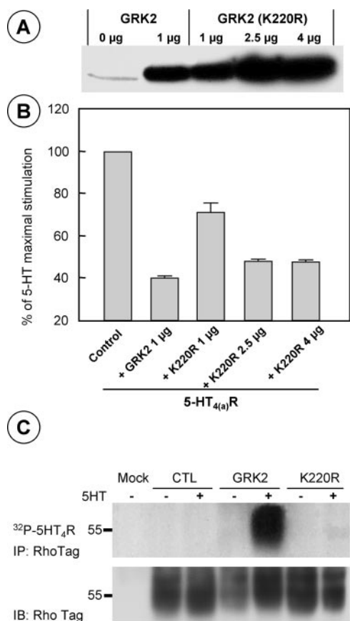
FIG. 5. GRK2 kinase activity is not required for 5-HT 4 R uncoupling. COS-7 cells were transiently transfected with 5-HT 4(a) R (100 ng of plasmid) with either GRK2 (1 \mu g) or different amounts of dominant-negative GRK2(K220R) (1–4 \mu g). A , the expression levels of transfected GRK2 and GRK2(K220R) were revealed by Western blotting of whole cell lysates 24 h after transfection. B , the effect of overexpression of GRK2 and GRK2(K220R) was tested for cAMP production in response to 30 \mu M 5-HT for 5 min in the presence of Ro 20-1724. Data are expressed as a percentage of the maximum cAMP response produced by 5-HT 4(a) R expressed alone. Basal and 5-HT-stimulated cAMP values were 32 \pm 4 and 177 \pm 6 pmol/well, respectively. ELISA were performed to quantify cell-surface receptor expression before and after agonist stimulation. Data represent the means \pm S.E. for three independent experiments. C , the phosphorylation state of 5-HT 4(a) R was studied following metabolic labeling with 32 P in the absence or presence of GRK2 or GRK2(K220R) overexpression. Cells transfected with 5-HT 4(a) R (1 \mu g of plasmid) alone or with either GRK2 (1 \mu g) or GRK2(K220R) (2.5 \mu g) were incubated (+) or not (–) with 10 \mu M 5-HT for 10 min. The receptor was purified by immunoprecipitation (IP) using anti-Rho tag monoclonal antibody. The identity of the bands was confirmed by Western blot analysis (immunoblotting (IB)) using mouse anti-Rho tag antibody. The autoradiograms shown are representative of three independent experiments. CTL, control.
