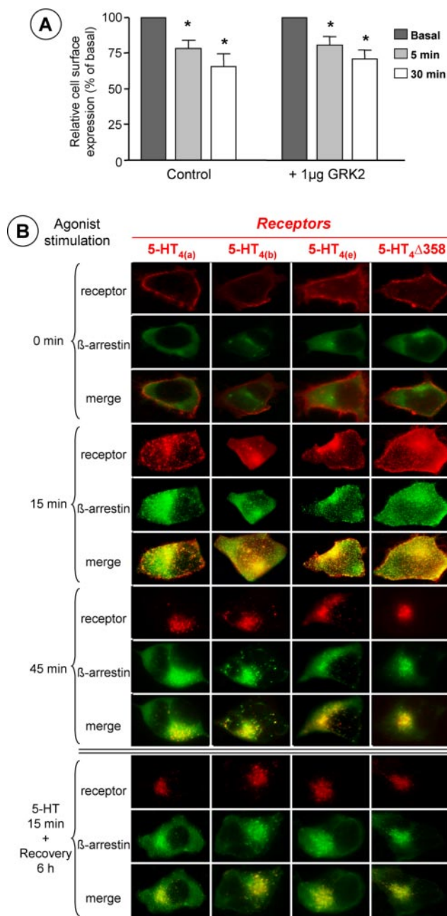
FIG. 6. Overexpression of GRK2 is not required for 5-HT 4 R endocytosis in HEK293 cells. Similar 5-HT 4 R/ \beta -arrestin endocytosis was observed, regardless of the 5-HT 4 R splice variant considered. A , cell-surface expression of HA-tagged 5-HT 4 R (100 ng of plasmid) transfected alone in HEK293 cells or in combination with 1 \mu g of cDNA encoding GRK2 was determined by ELISA before and after stimulation with 5-HT (10 \mu M) for 5 and 30 min as described under “Experimental Procedures.” Data represent the means \pm S.E. of four independent experiments. *, p < 0.01 (significantly different from the corresponding cells before 5-HT treatment). B , HEK293 cells were transiently cotransfected with 600 ng of c-Myc-tagged 5-HT 4(a) R, 5-HT 4(b) R, or 5-HT 4(e) R splice variant or \Delta 358 mutant in combination with 1 \mu g of GRK2 and 0.3 \mu g of \beta -arrestin-2-YFP. Intact cells were immunostained with anti-c-Myc antibody before activation of 5-HT 4 R. The upper panels show the distribution of \beta -arrestin-2-YFP and c-Myc-tagged 5-HT 4 R splice variants either before (0 min; control) or after (15 and 45 min) addition of 5-HT (30 \mu M) to the culture medium. The lower panels show cells that were stimulated for 15 min with agonist and then extensively washed and subjected to an additional incubation in agonist-free medium for 6 h. Cells were fixed either after a stimulation period in the presence of the agonist or after a period of recovery in agonist-free medium. Immunoreactivity was revealed with Alexa Fluor 594-conjugated secondary antibodies. Fluorescence microscopy was then used to visualize the redistribution of antibody-labeled receptors and \beta -arrestin-2-YFP. Note that the majority of vesicles containing internalized 5-HT 4 R also contained \beta -arrestin-2-YFP.
