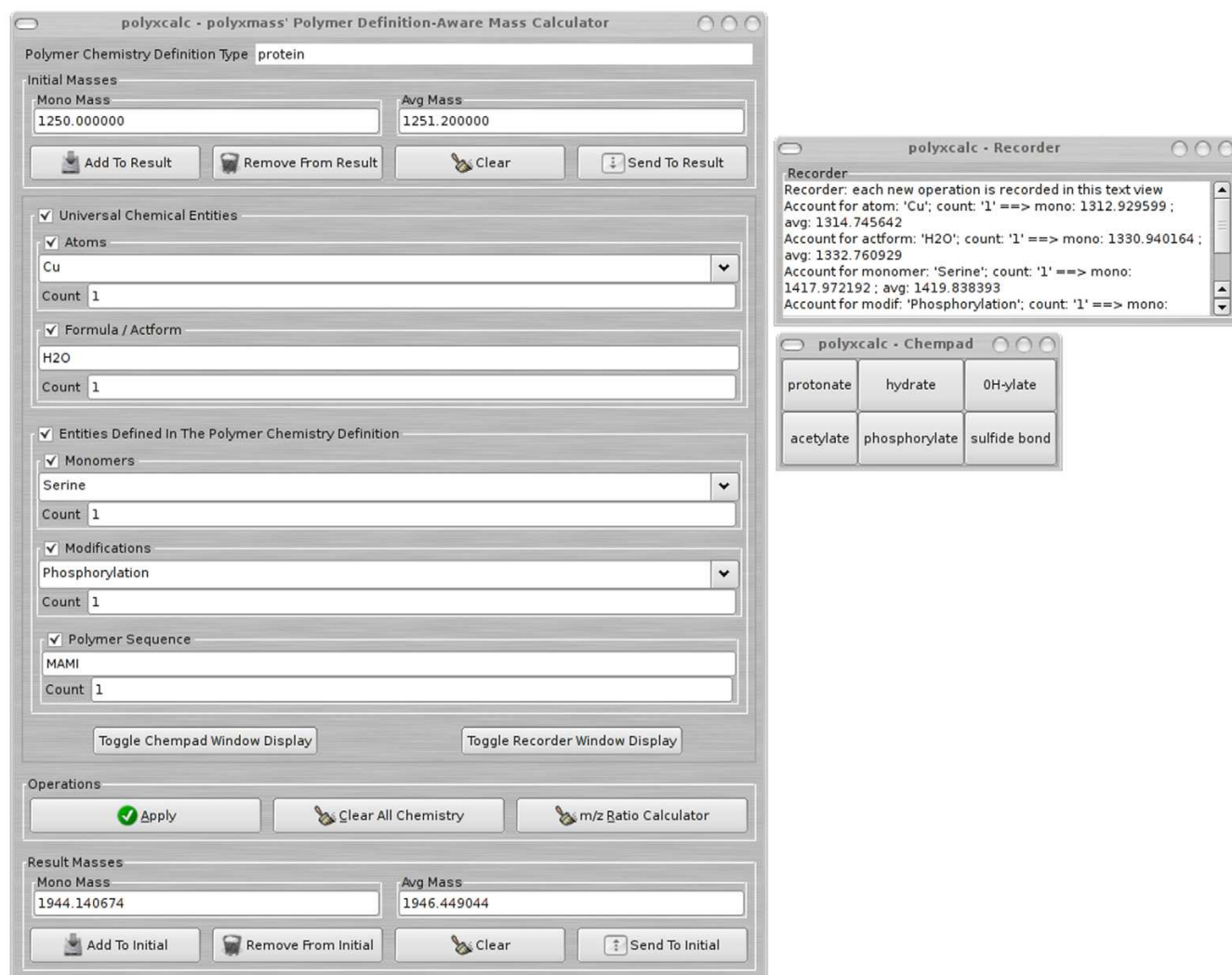
Figure 4 The polyxcalc programmable mass calculator. The mass calculator is polymer chemistry definition-aware, and in this figure it is represented pre-loaded with the "protein" polymer chemistry definition (top of the left window). When, upon opening of the calculator, a polymer chemistry definition is loaded, its chemical entities (monomers and chemical modifications, as shown) become available in the calculator's widgets; otherwise only atoms and formulas can be used. The calculator is programmable, and a simple syntax allows the definition of the layout of a "chemical pad" to perform quick chemical calculation tasks in the calculator.
