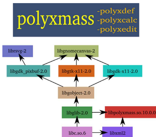
Figure 1 Software dependencies of the GNU polyxmass project. The libpolyxmass library has few dependencies while the polyxmass program has more dependencies due to its use of a number of graphical libraries for the window system and the graphical rendering of the polymer sequence.
