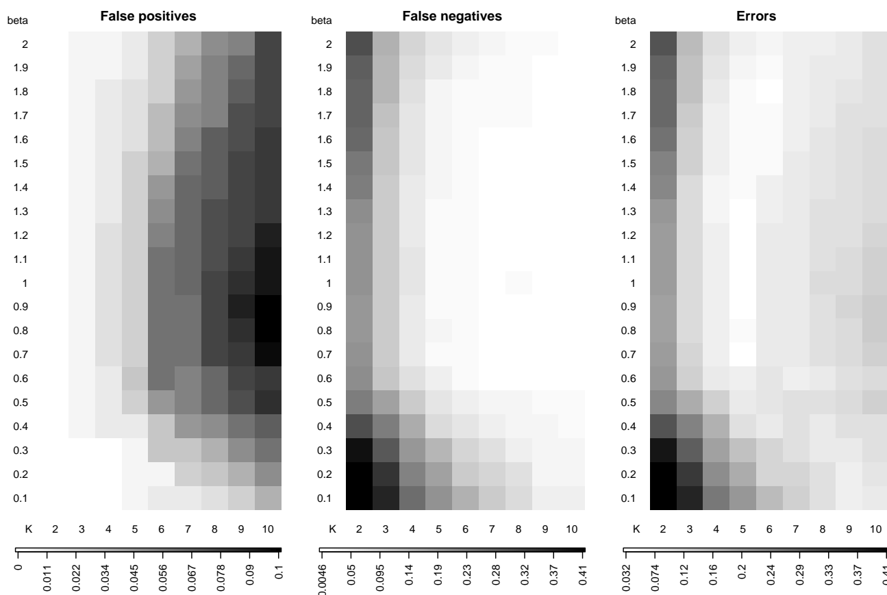
Figure 10 Comparison between qualitative assessment and segmentation results with various ( K , \beta ) – bladder cancer data set. The segmentation algorithm is run with K \in \{2, \dots, 10\} (x axis) and \beta \in \{0.1, 0.2, \dots, 2.0\} (y axis) and compared with the expert assessment of the breast cancer data set. (a) False positive rate; (b) False negative rate; (c) Total error rate.
