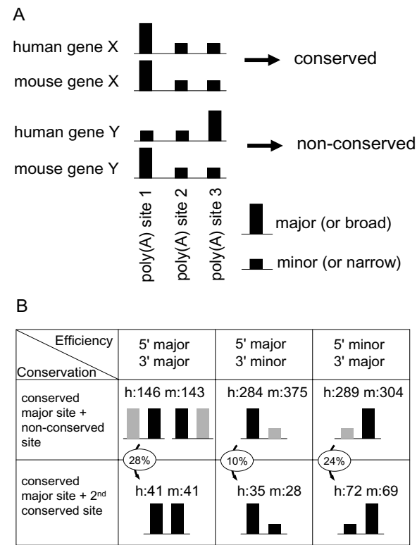
Figure 8 Spatial efficiency/specificity patterns and conservation. (A) Definition of spatial efficiency/specificity patterns. Ortholog gene pairs with identical numbers of conserved polyadenylation sites are considered. A conserved pattern is defined as a series of sites between two orthologous genes, where each site bares the same properties (major/minor or broad/narrow) as its orthologous counterpart (e.g. gene X). All other patterns are defined as non-conserved (e.g. gene Y). (B) Relationship between tandem poly(A) site spatial patterns and conservation. The first row shows different patterns in which one major site is conserved. The second row shows different patterns in which two sites are conserved. Numbers of human genes ("h") and mouse genes ("m") displaying each pattern are shown. Circled numbers indicate ratio of patterns in second row over patterns in first row.
