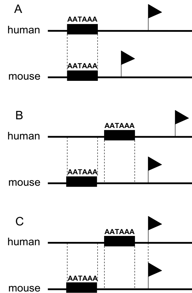
Figure 1 Definition of conserved and non-conserved polyadenylation sites. Cleavage sites are shown by flags and polyadenylation signals are shown by black squares. (A) sites are within 30 bp of each other and aligned associated signals: conserved; (B) sites are within 30 bp of each other, however, their associated signals are not aligned: non conserved; (C) although the sites themselves are aligned, their signals are not: non conserved.
