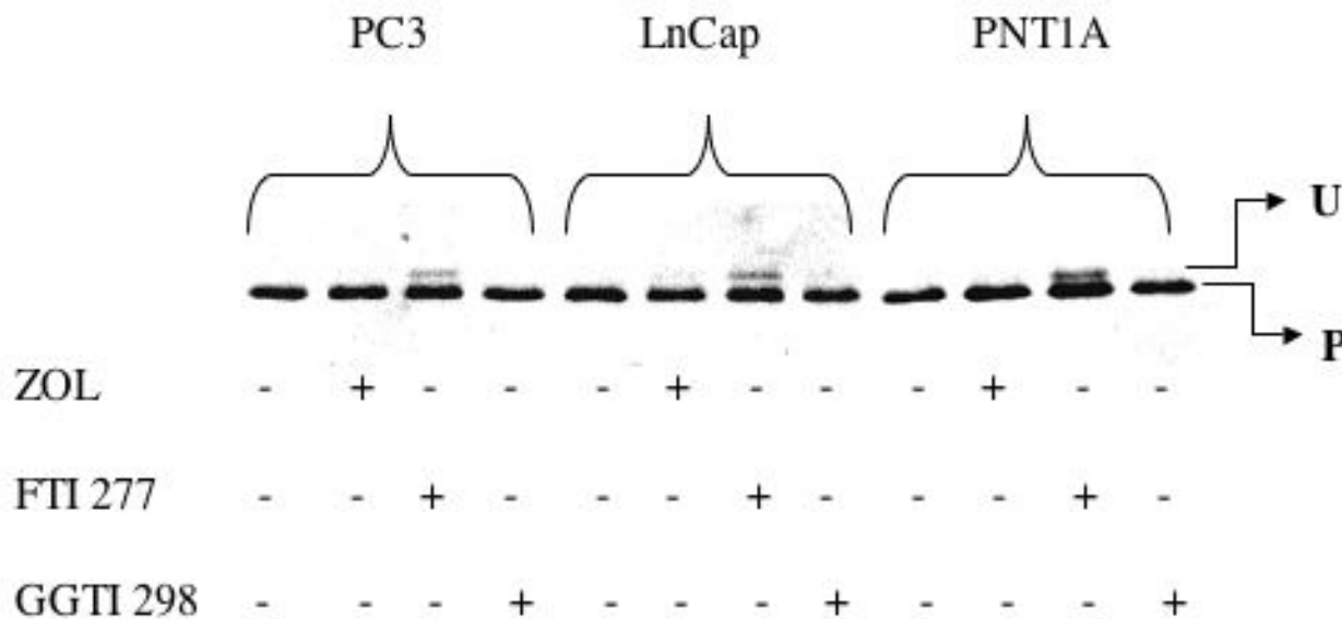
Figure 3 Effect of zoledronate on farnesylation status of HDJ2. Prostatic cells were treated for 48 h with ZOL (20 μM), lysed in hot (90°C) SDS (1%) and analyzed by Western blot.
